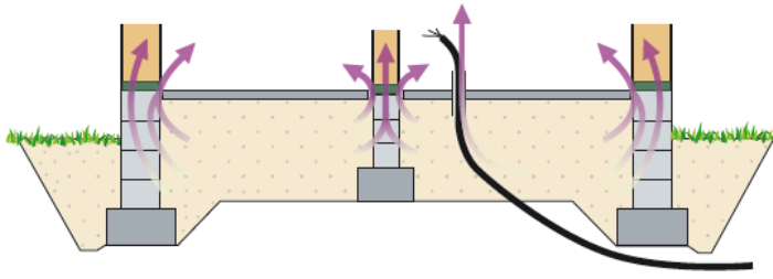
Figure 1. Entry routes of soil air in a Finnish slab-on-ground foundation. The foundation wall is constructed of permeable light-weight concrete blocks.
